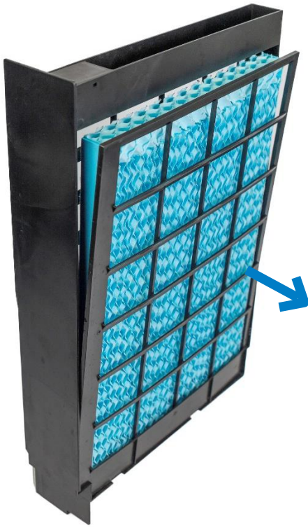
Fig. 4.5.2: Removing the grid of the filter carrier
